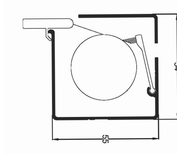
cassette with tube, spring and reflector foil
